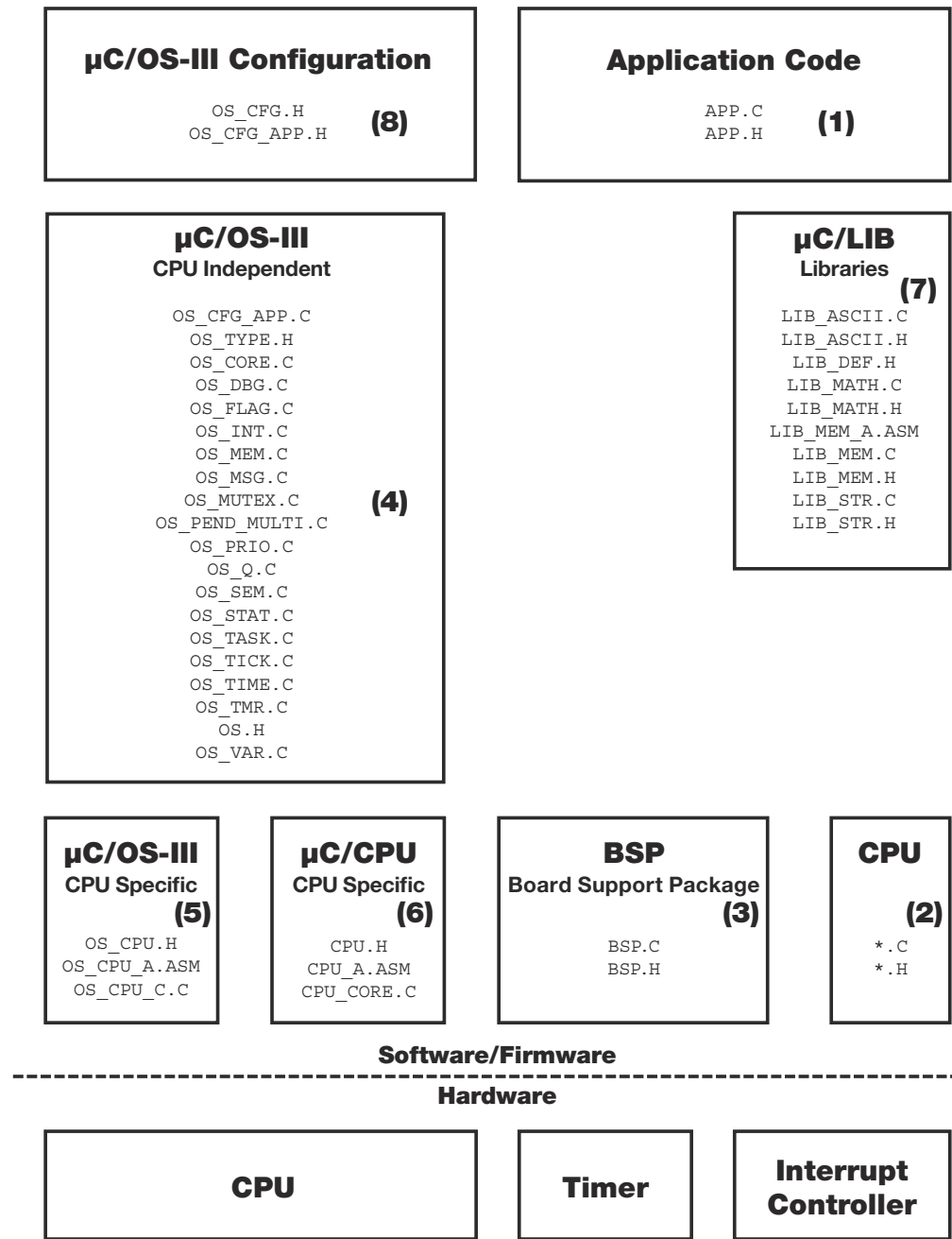
Figure 2-1 μC/OS-III Architecture
