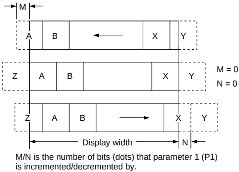
Figure 21. Horizontal scrolling
