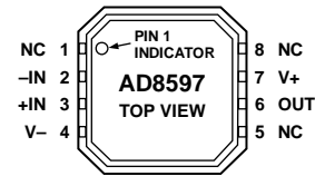
Figure 2. AD8597 8-Lead LFCSP (CP-8-2)
