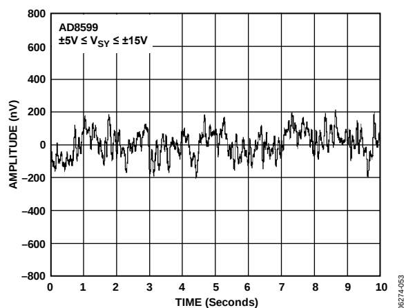
Figure 54. Peak-to-Peak Noise
