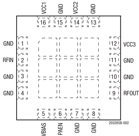
Figure 2. SKY66294-11 Pinout (Top View)
