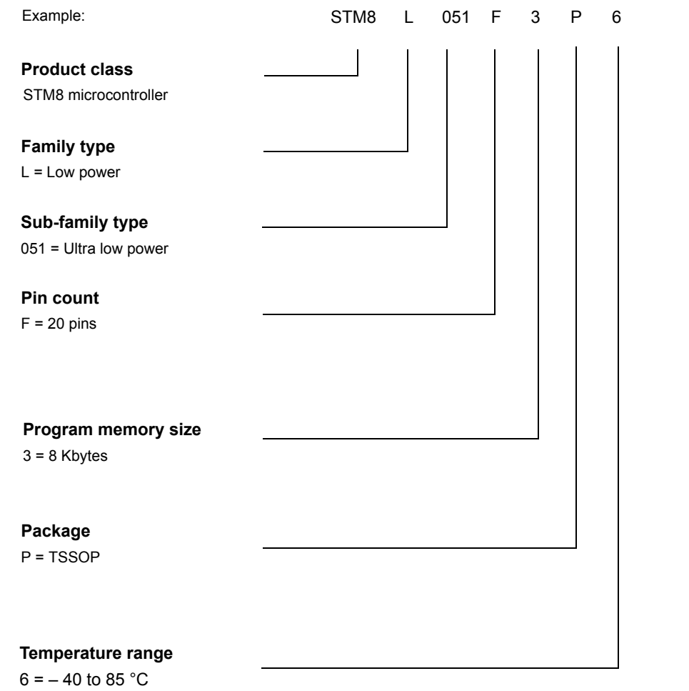
Figure 40. Low density value line STM8L051F3 ordering information scheme
