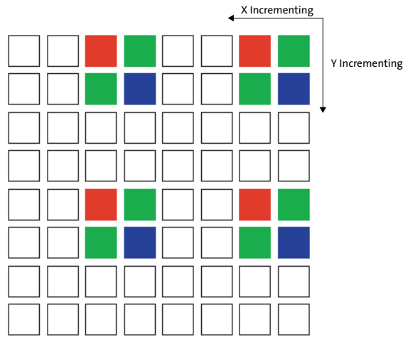
Figure 18: Pixel Readout (Column and Row Skipping)
