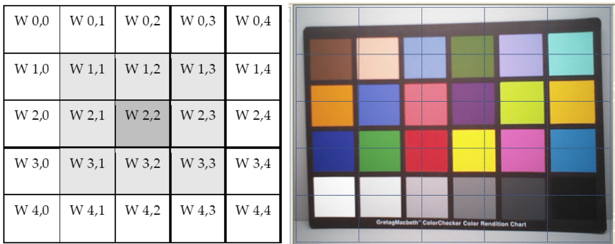
Figure 26: 5 x 5 Grid
