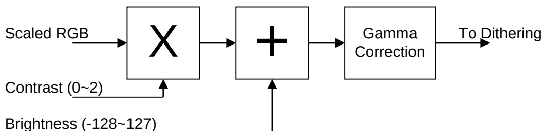
Figure 9 Brightness, Contrast & Gamma Correction block diagram
