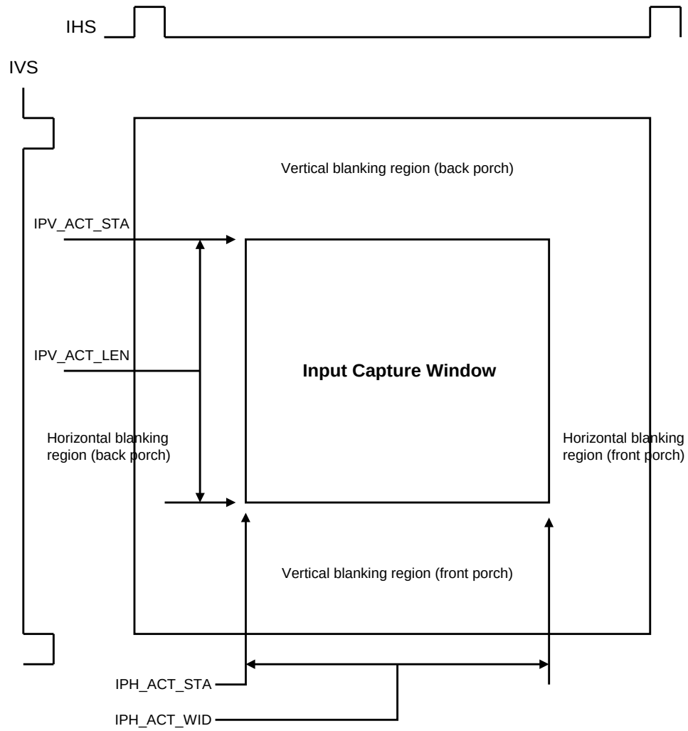
Figure 5 Input Capture Window
