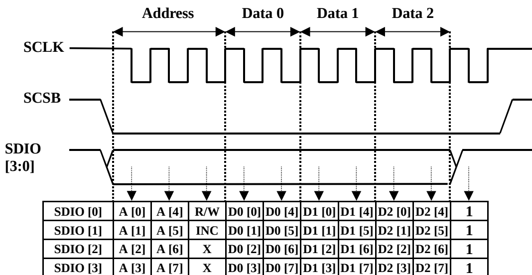
Figure 16 Parallel Port Timing
