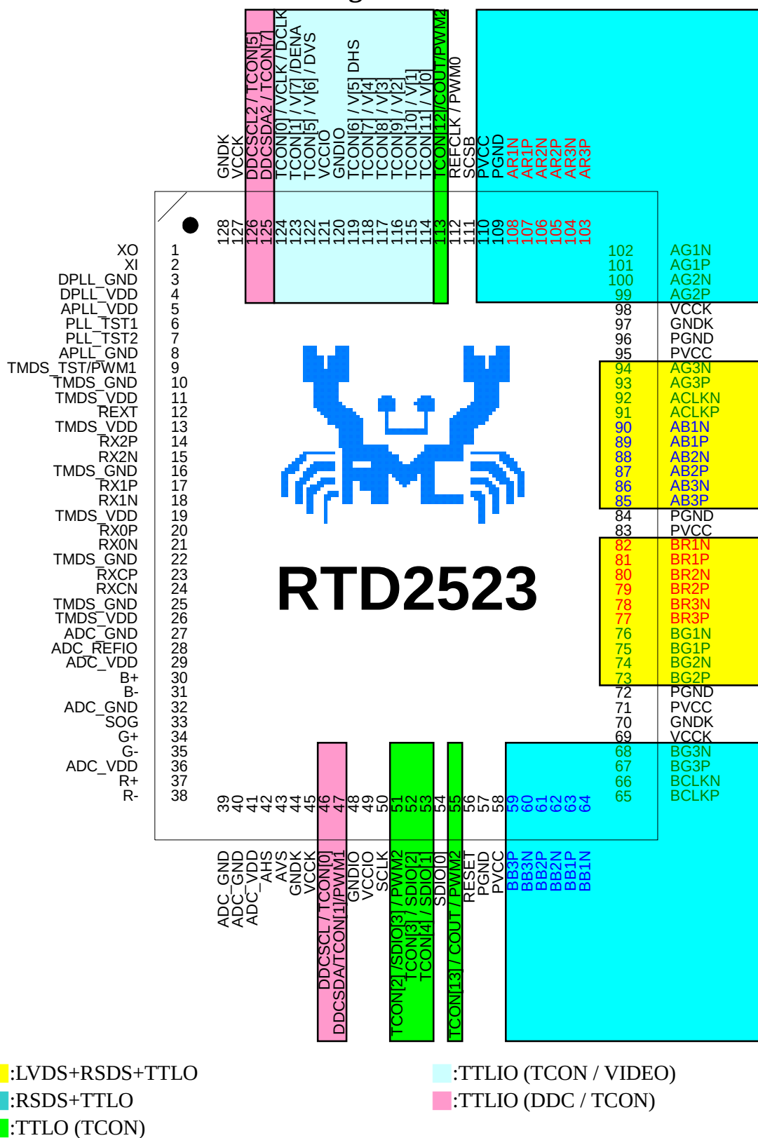
Figure 1 Pin-Out Diagram ( 6-bit Dual RS232C )
