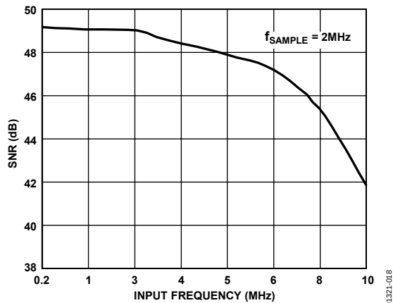
Figure 18. SNR vs. Input Frequency on the AD7825
