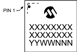
48-Lead UQFN (6x6x0.5 mm)
