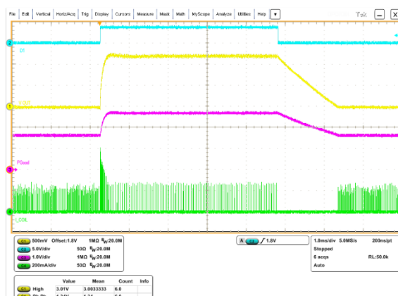
Figure 10. V_{OUT} change, 1.8 V to 3.3 V to 1.8 V, I_{OUT}=5\text{ mA}
