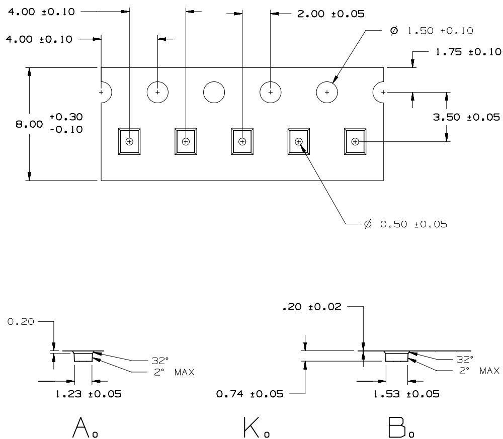
Figure 26. Flip-Chip 8 (1.14x1.44 mm) tape orientation
