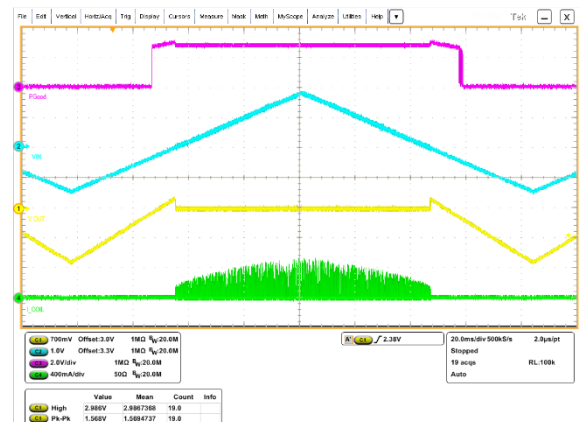
Figure 9. 100% mode, V_{OUT} = 3.0\text{ V}
