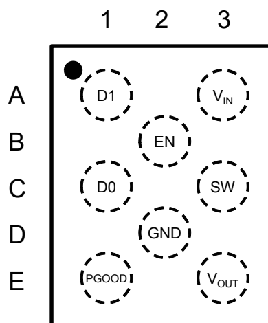
Figure 2. Flip-Chip8 package
