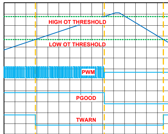
FIGURE 26. OVER-TEMPERATURE FAULT
