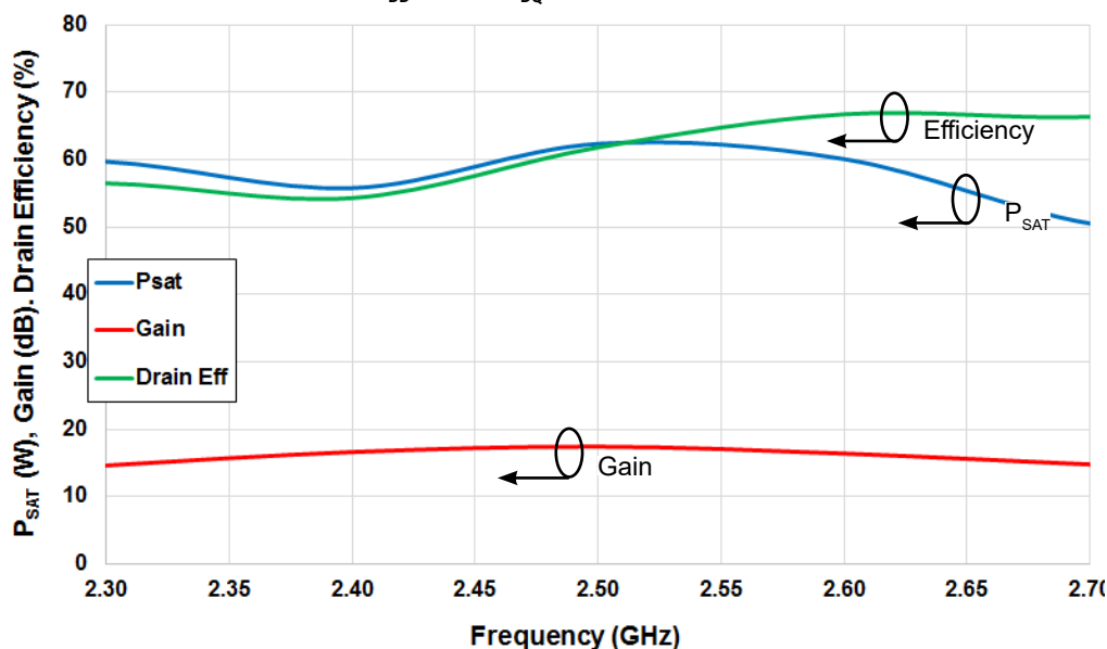
Figure 2. - Gain, Efficiency, and Output Power vs Frequency measured in Amplifier Circuit CG2H40045F-AMP
