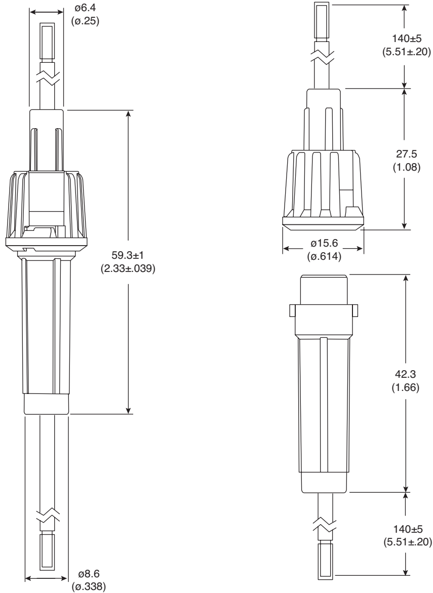
DIMENSIONS: mm (in.)
