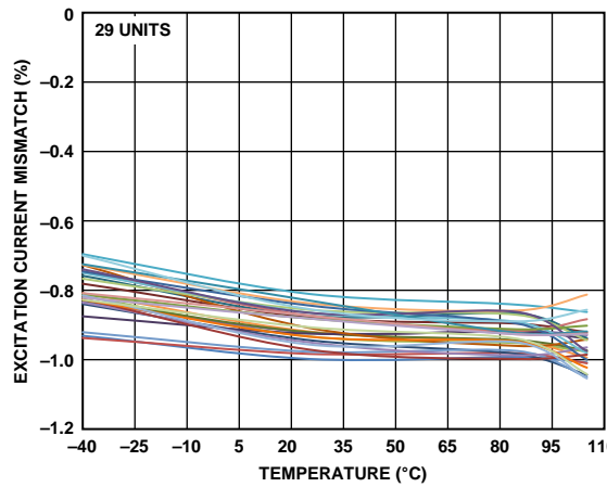
Figure 33. Excitation Current Drift Matching (500 µA)
