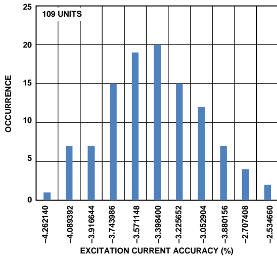
Figure 30. IOUTx Current Initial Accuracy Histogram (500 μA)
