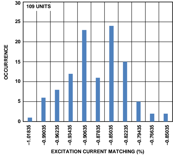
Figure 31. IOUTx Current Initial Matching Histogram (500 μA)
