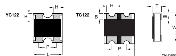
Fig. 4 YC/TC122 series chip resistors dimension
