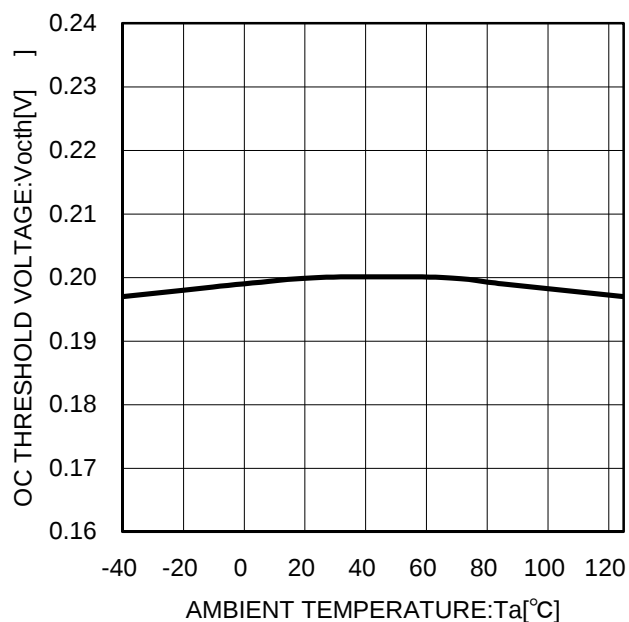
Figure 10. Overcurrent threshold voltage vs. temperature characteristics
