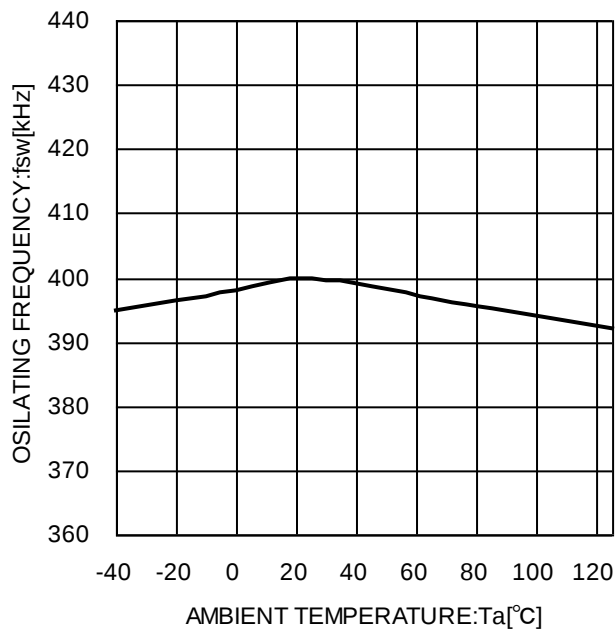
Figure 7. Oscillation frequency vs. temperature characteristics
