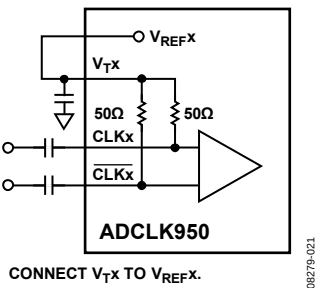
Figure 21. AC-Coupled Input Termination, Such as LVDS and LVPECL
