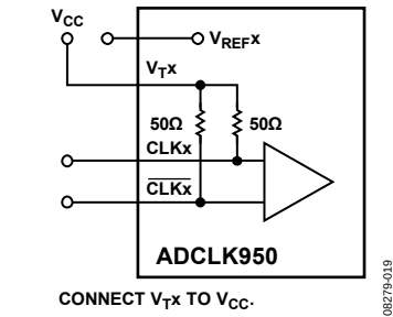
Figure 19. DC-Coupled CML Input Termination
