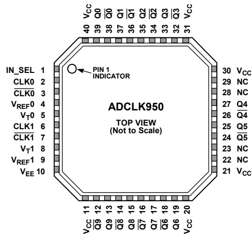
Figure 2. Pin Configuration
