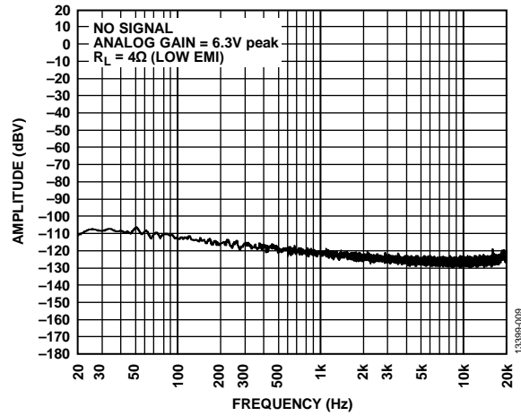
Figure 11. Amplitude vs. Frequency, No Signal, Analog Gain = 6.3 V peak
