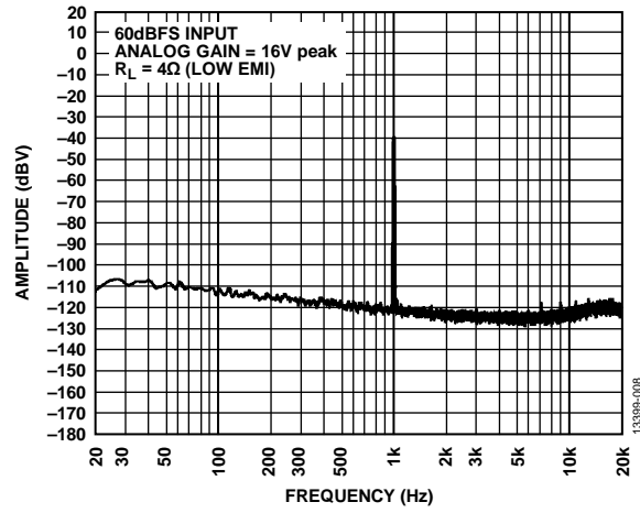
Figure 10. Amplitude vs. Frequency, 60 dBFS Input, Analog Gain = 16 V peak
