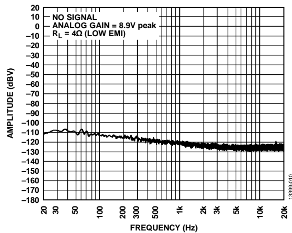
Figure 12. Amplitude vs. Frequency, No Signal, Analog Gain = 8.9 V peak
