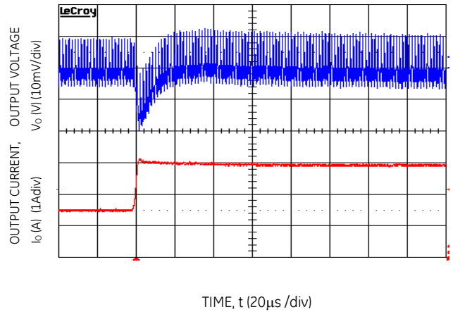
Figure 16. Transient Response to Dynamic Load Change from 50% to 100% at 12V in , C out -1x47uF+1x330uF, C Tune -10nF & R Tune -261
