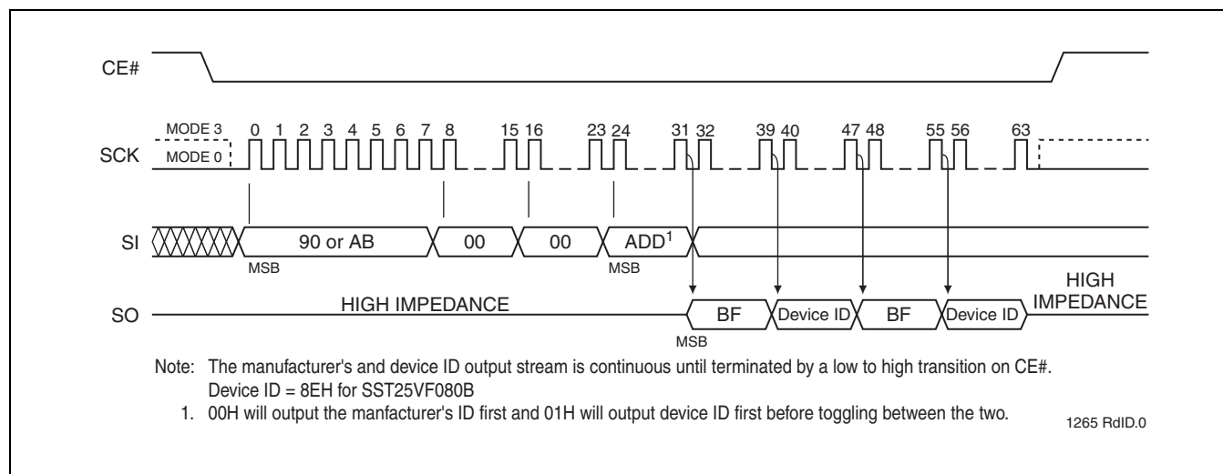
FIGURE 21: Read-ID Sequence
