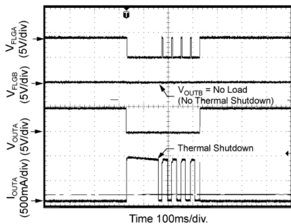
Independent Thermal Shutdown, Out A
