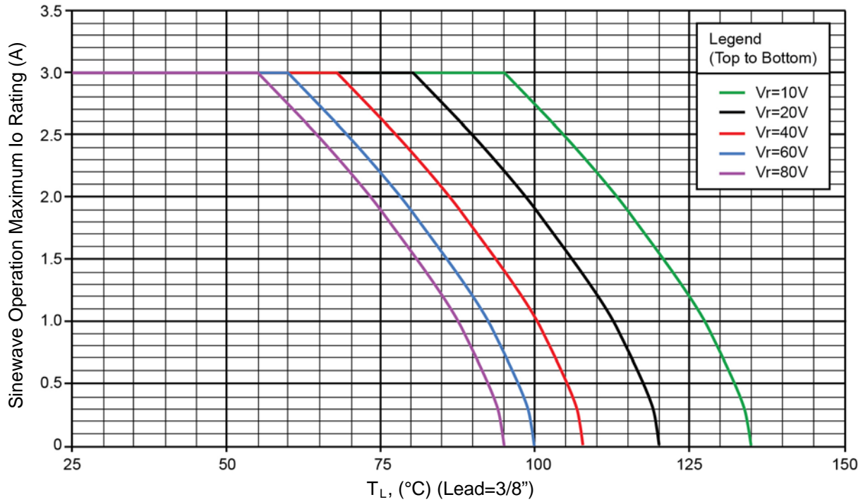
FIGURE 4 Temperature current derating for 1N6864
