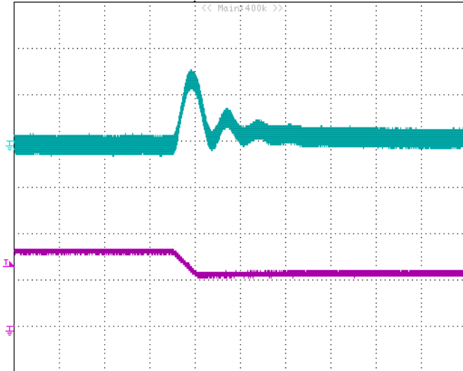
Figure 8: Output voltage response to step-change in load current (75%-50% of I_o max; di/dt = 0.1A/\mu s , V_{in}=48V ). Load cap: 300\mu F , electrolytic capacitor ; 10\mu F , tantalum capacitor and 1\mu F ceramic capacitor. Top Trace: V_{out} (200mV/div, 200us/div); Bottom Trace: I_o (20A/div, 200us/div). Scope measurement should be made using a BNC cable (length shorter than 20 inches). Position the load between 51 mm to 76 mm (2 inches to 3 inches) from the module..
