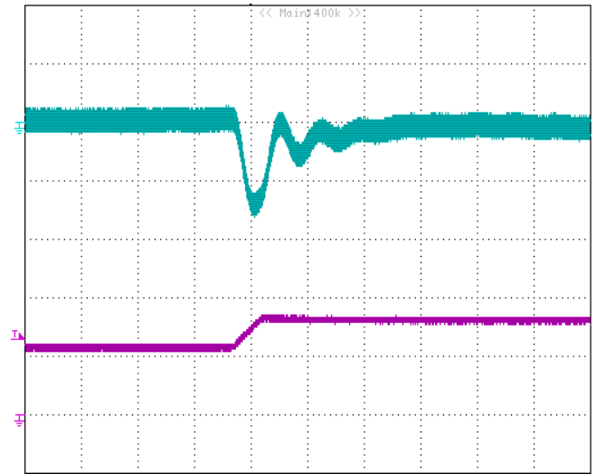
Figure 9: Output voltage response to step-change in load current (50%-75% of I_o max; di/dt = 0.1A/\mu s , V_{in}=48V ). Load cap: 300\mu F , electrolytic capacitor ; 10\mu F , tantalum capacitor and 1\mu F ceramic capacitor. Top Trace: V_{out} (200mV/div, 200us/div); Bottom Trace: I_o (20A/div, 200us/div). Scope measurement should be made using a BNC cable (length shorter than 20 inches). Position the load between 51 mm to 76 mm (2 inches to 3 inches) from the module..
