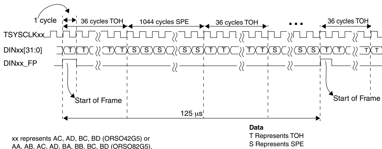
Figure 18. Transmit SONET Mode
