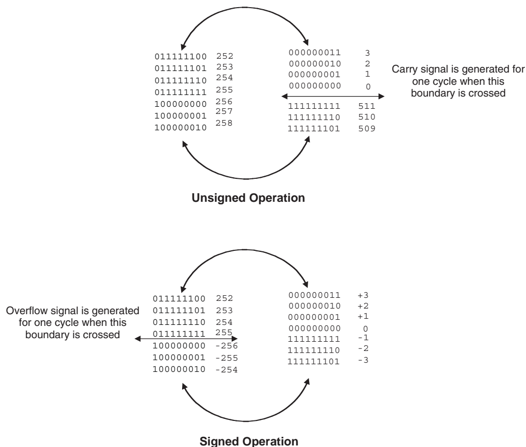
Figure 2-24. Accumulator Overflow/Underflow
