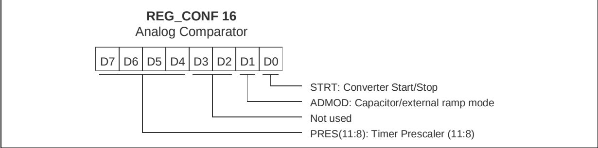
Figure 7.5 Configuration Register 16
