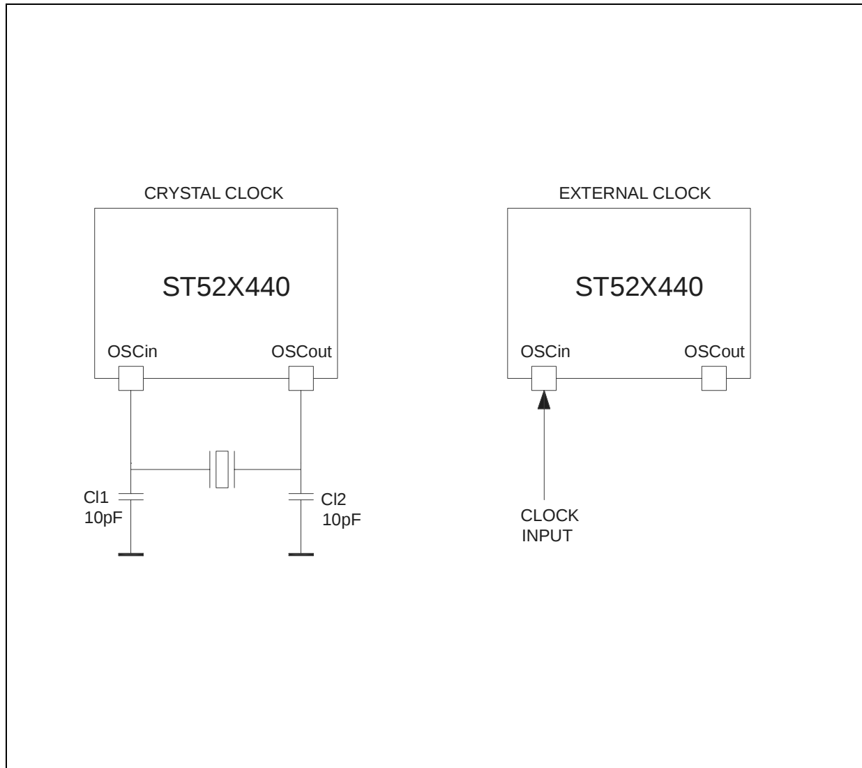
Figure 5.1 Oscillator Connections
