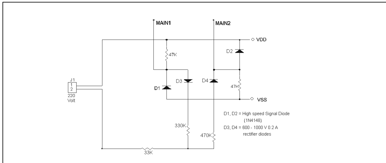
Figure 10.6 Burst Mode Zero Crossing Circuit
