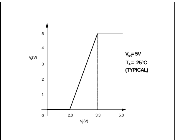
Figure 11.11 Port B pins CMOS-level input
