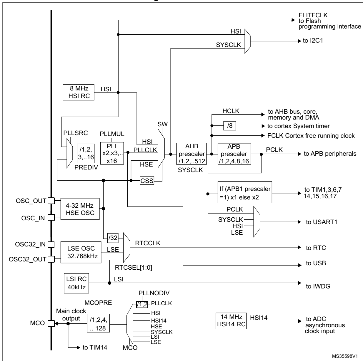
Figure 2. Clock tree
