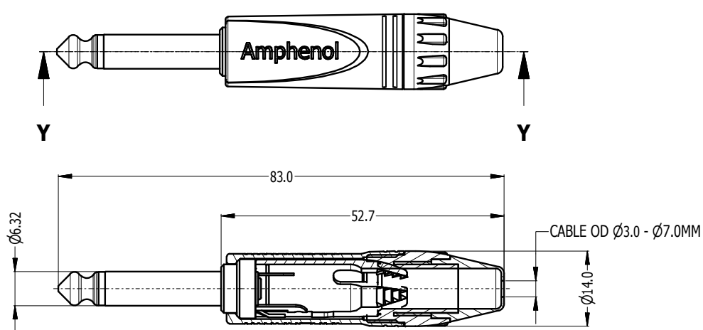
SECTION Y-Y
