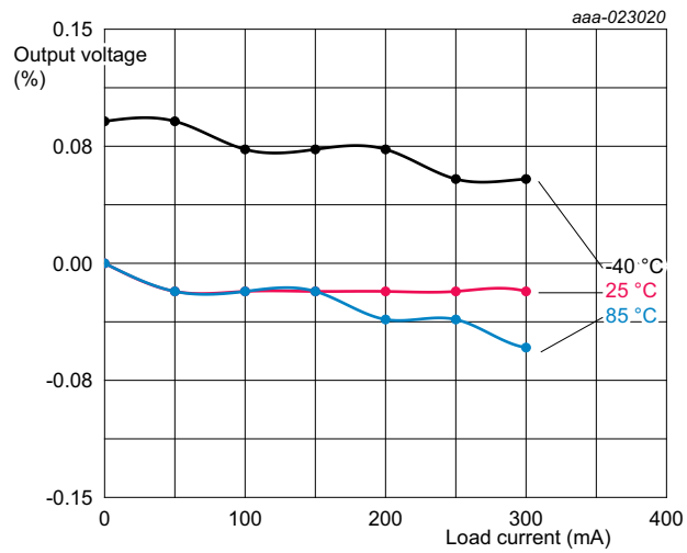
Fig 8. Output regulation vs load current and temp ( V_{IN} = 3.6 V)
