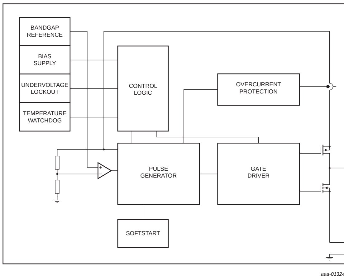
Fig 1. Block diagram
