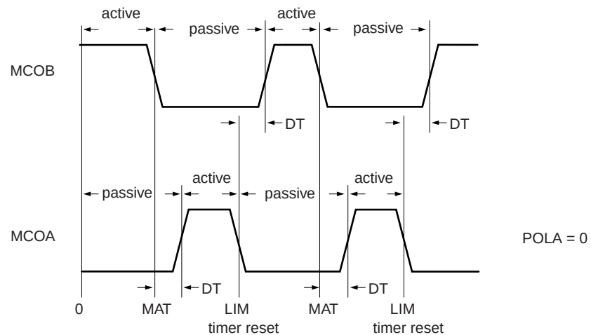
Fig 148. Edge-aligned PWM waveform with dead time, POLA = 0
