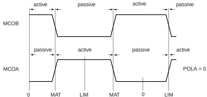
Fig 147. Center-aligned PWM waveform without dead time, POLA = 0
