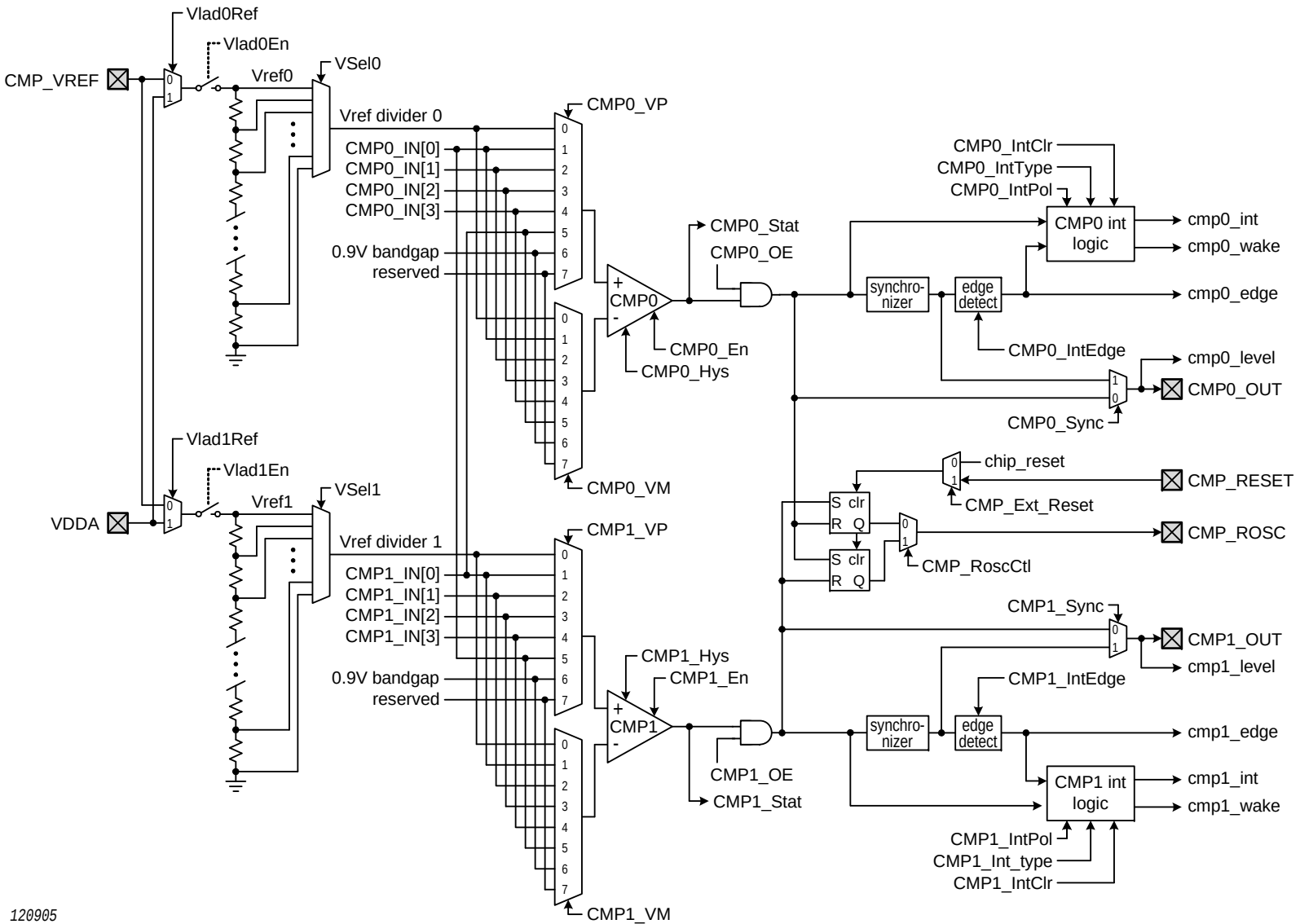
Fig 163.Comparator block diagram
