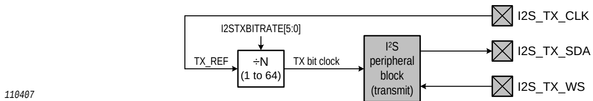
Fig 128. Typical transmitter slave mode
