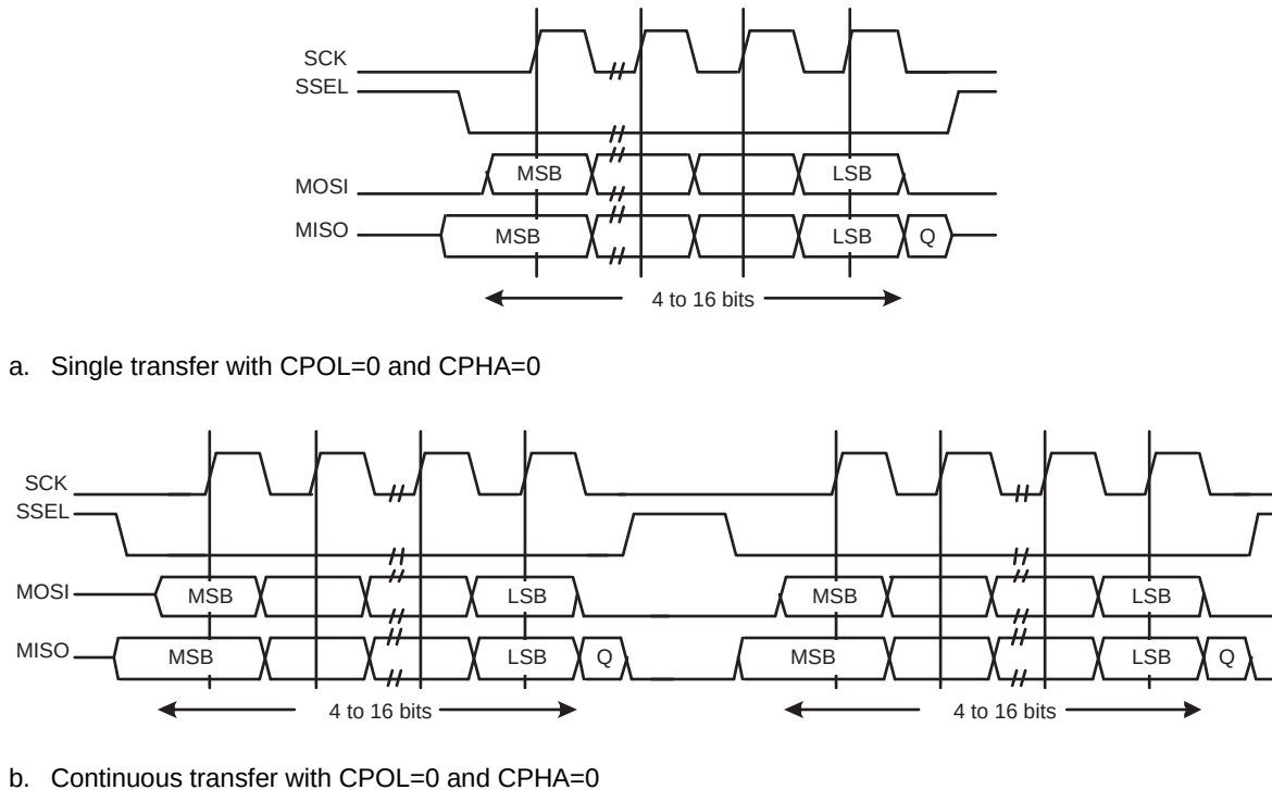
Fig 101. SPI frame format with CPOL=0 and CPHA=0 (a) Single and b) Continuous Transfer)
