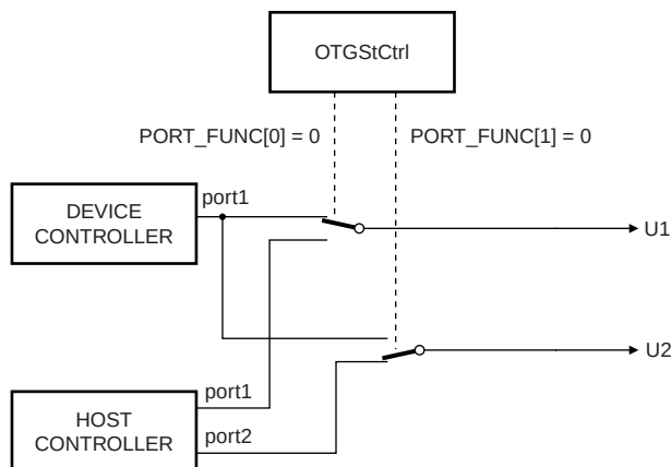
Fig 53. Port selection for PORT_FUNC bit 0 = 0 and PORT_FUNC bit 1 = 0
