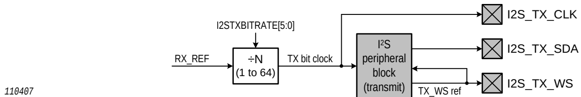
Fig 126. Transmitter master mode sharing the receiver reference clock
