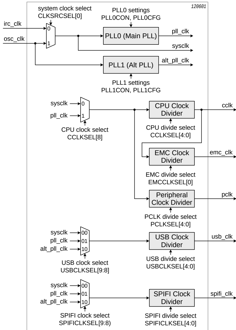
Fig 4. Clock generation
