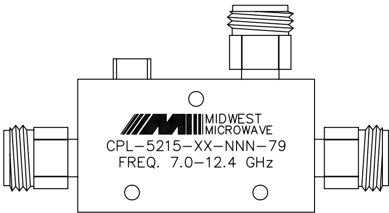
BACKSIDE MARKING
