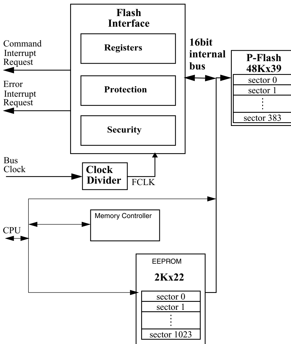
Figure 30-1. FTMRG192K2 Block Diagram
