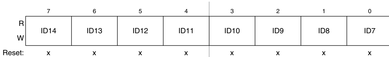
Figure 18-28. Identifier Register 2 (IDR2) — Extended Identifier Mapping
