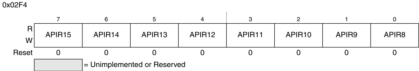
Figure 10-20. Autonomous Periodical Interrupt Rate High Register (CPMUAPIRH)
