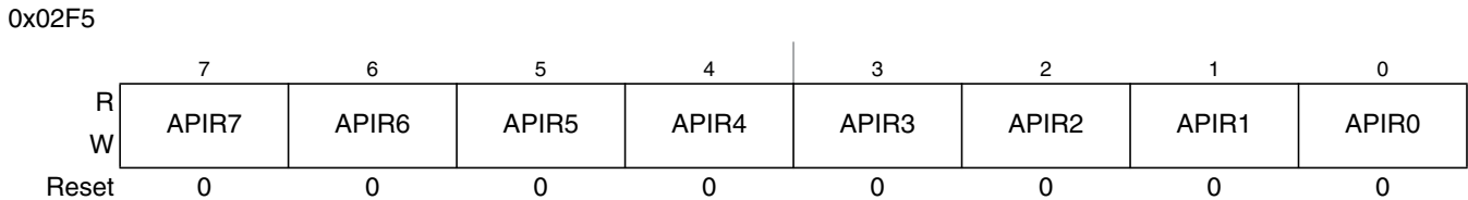
Figure 10-21. Autonomous Periodical Interrupt Rate Low Register (CPMUAPIRL)
