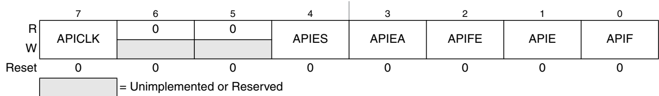
Figure 10-17. Autonomous Periodical Interrupt Control Register (CPMUAPICTL)
