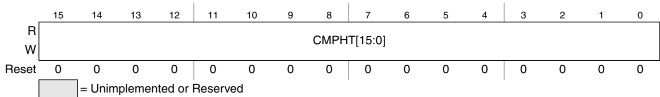
Figure 16-13. ATD Compare Higher Than Register (ATDCMPHT)
