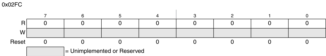
Figure 10-29. Reserved Register CPMUTEST2
