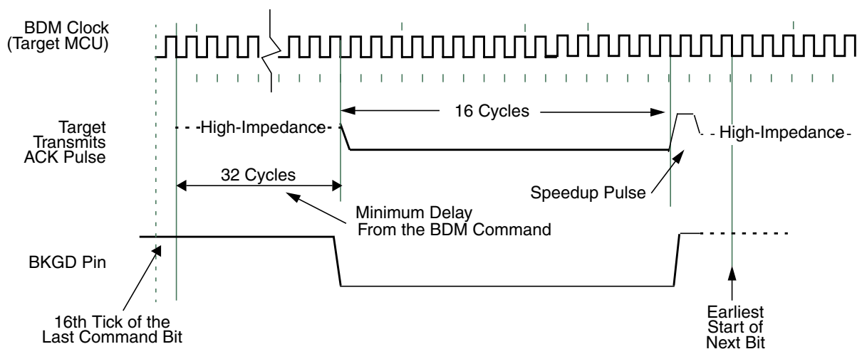
Figure 7-10. Target Acknowledge Pulse (ACK)
