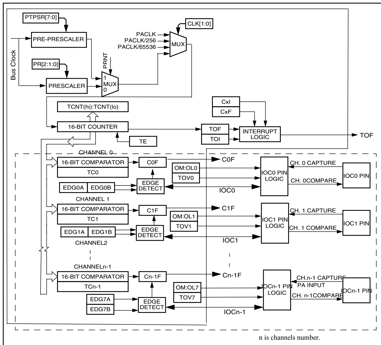
Figure 22-22. Detailed Timer Block Diagram
