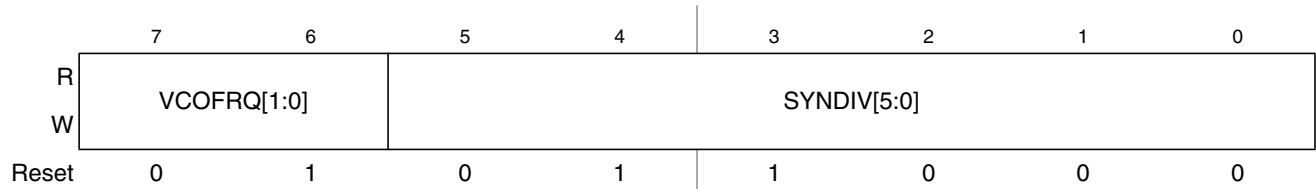
Figure 10-4. S12CPMU Synthesizer Register (CPMUSYNR)
