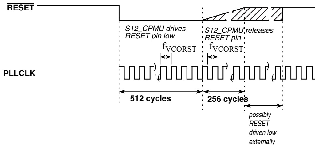
Figure 10-34. RESET Timing
