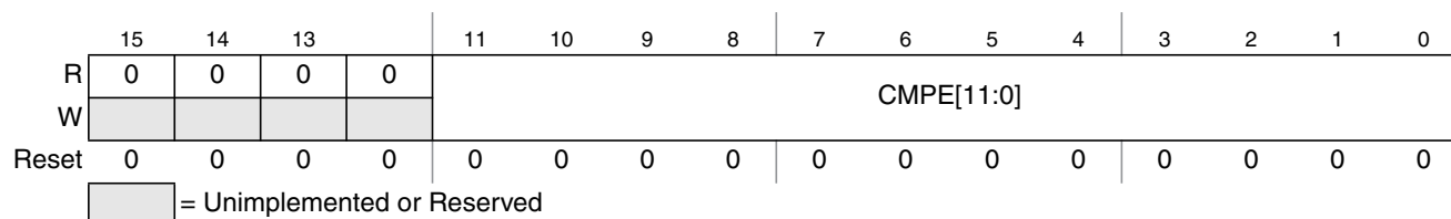
Figure 13-10. ATD Compare Enable Register (ATDCMPE)
