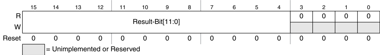
Figure 13-14. Left justified ATD conversion result register (ATDDR n )
