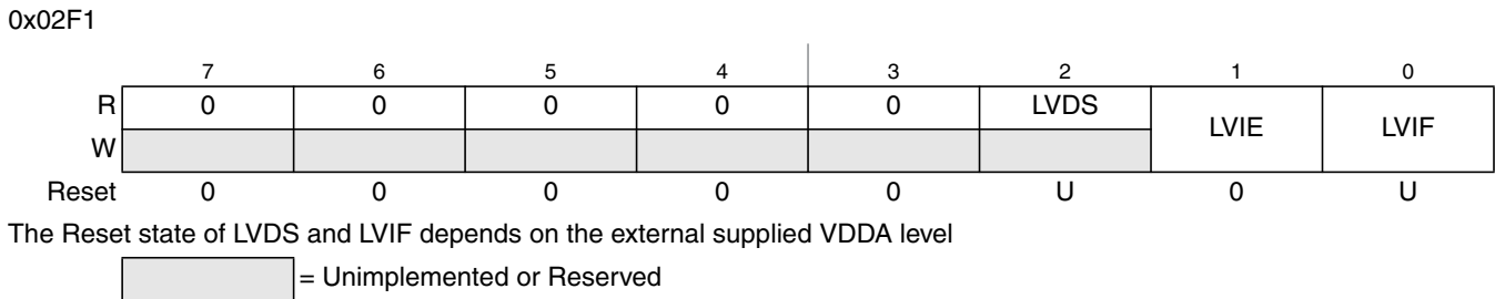
Figure 10-16. Low Voltage Control Register (CPMULVCTL)
