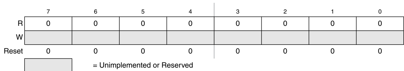
Figure 24-22. Flash Reserved5 Register (FRSV5)
