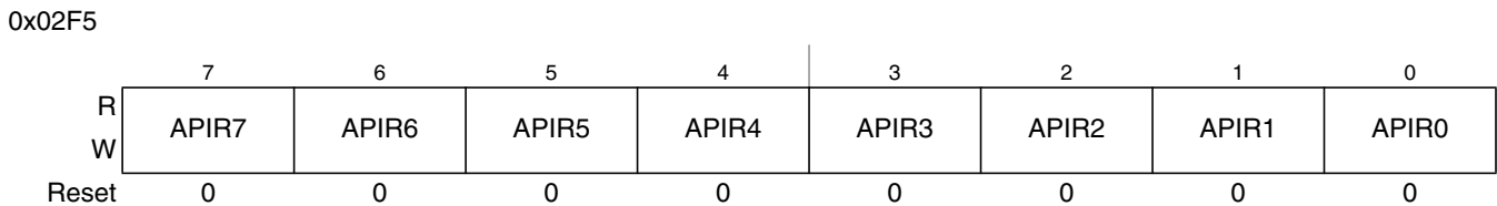
Figure 10-21. Autonomous Periodical Interrupt Rate Low Register (CPMUAPIRL)
