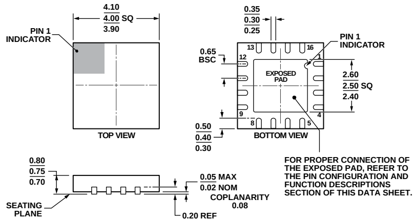
Figure 48. 16-Lead Lead Frame Chip Scale Package [LFCSP_WQ] 4 mm × 4 mm Body, Very Very Thin Quad (CP-16-26) Dimensions shown in millimeters
