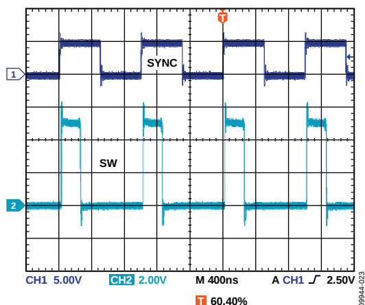
Figure 23. ADP2164 Synchronized to 1 MHz, in Phase
