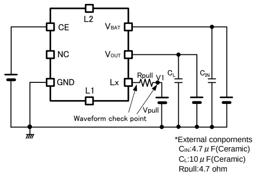
<Test Circuit No.⑧>
