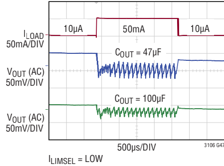
5V V_{IN} to 1.8V V_{OUT} Load Step 10 \mu A to 50mA
