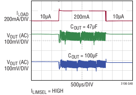
5V V_{IN} to 1.8V V_{OUT} Load Step 10 \mu A to 200mA
