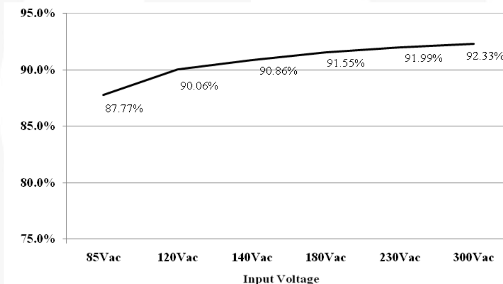
Figure 17. System Efficiency
