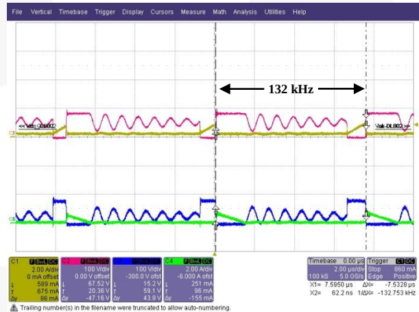
Figure 64. 10% Load [2 us/div]
