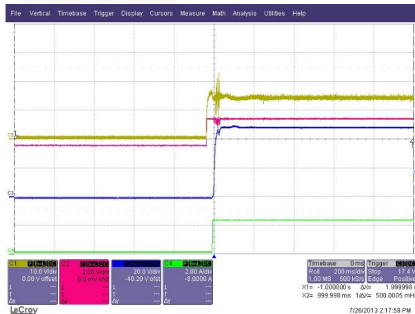
Figure 35. PS-ON
