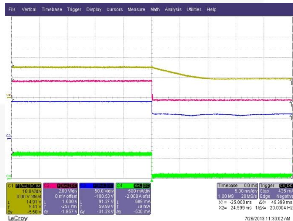
Figure 24. PS-OFF [5 ms/div]
