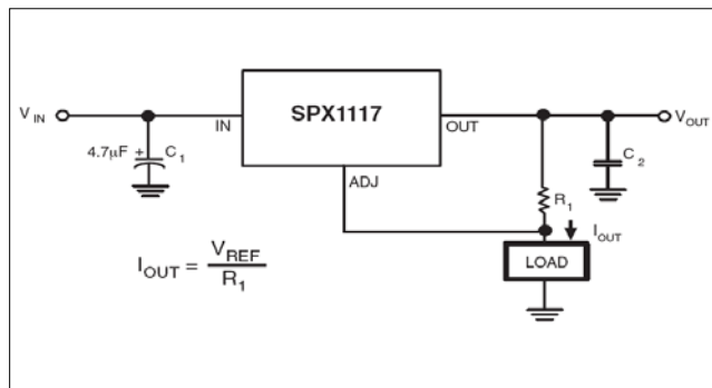
Fig. 21: Current Source
