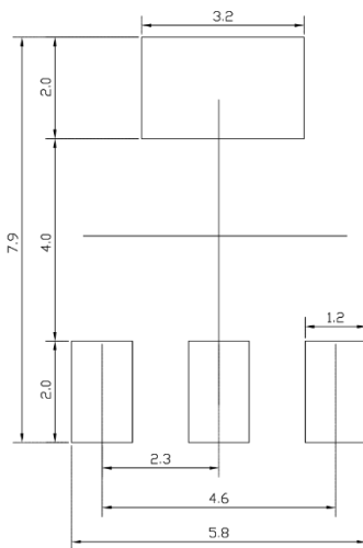
TYPICAL RECOMMENDED LAND PATTERN
