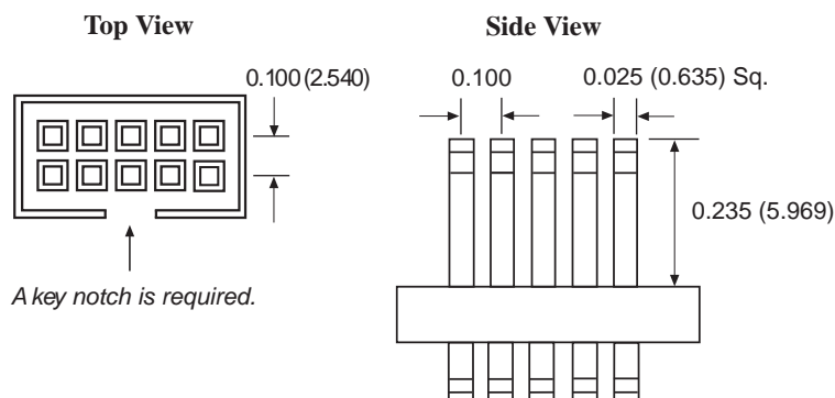
Figure 5. 10-Pin Male Header Dimensions - Inches and Millimeters
