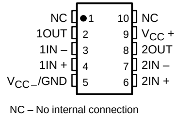
TLC2262M, TLC2262AM . . . U PACKAGE (TOP VIEW)
