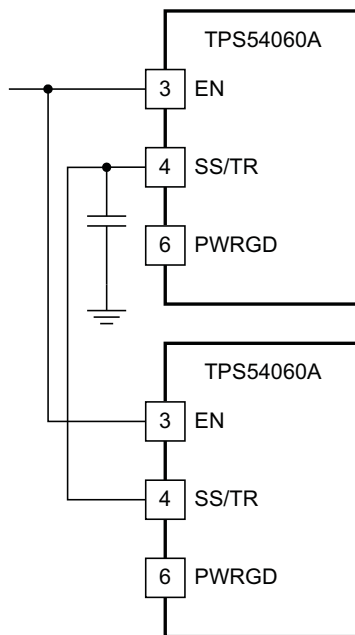
Figure 34. Schematic for Ratiometric Start-Up Sequence
