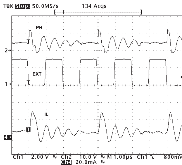
Figure 46. Plot of Synchronizing in PSM
