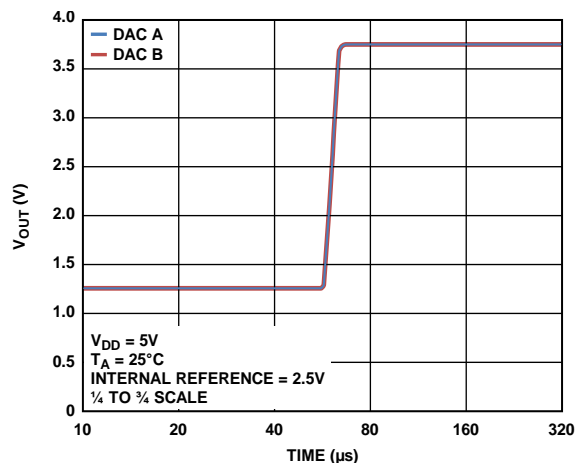
Figure 29. Settling Time
