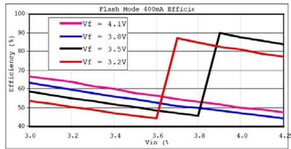
Fig. 7: Efficiency vs Supply Voltage C_{IN}=2.2\mu F , C_{FC}=0.47\mu F , C_{OUT}=1\mu F
