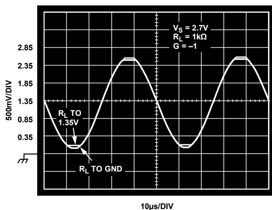
Figure 40. Output Swing
