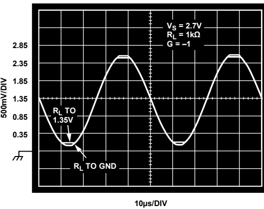
Figure 40. Output Swing
