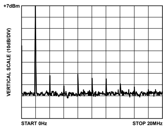
Figure 53. THD of Low Distortion Line Driver at 2 MHz
